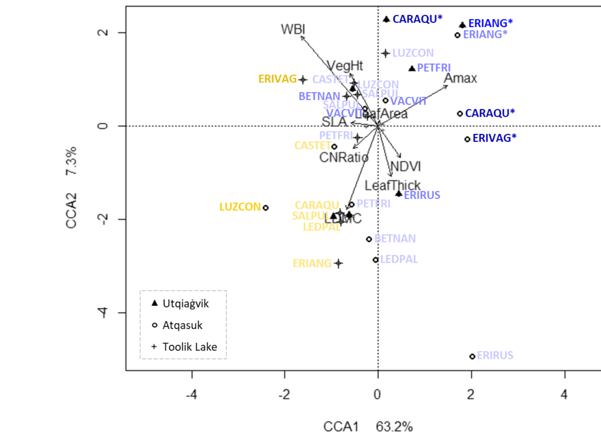
Fig 3: Canonical correspondence analysis (CCA) of average cover values from each year of sampling and average trait values for 12 Arctic plant species. Species codes follow the pattern of Genus species = GENSPE. Proportions of unconstrained variation explained are expressed on the axes. Results from post hoc analysis (999 permutations) indicate that the model (p<0.01) and first axis (p<0.01) are significant. Species in blue increased in cover from the first to last sampling with darker shades increasing the most and lighter shades increasing the least. Species in yellow decreased in cover from the first to last sampling. Species that significantly increased (repeated measures ANOVA) are indicated with an asterisk (*).
