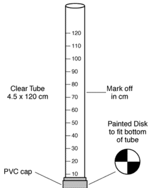
Figure 12 Turbidity Tube
