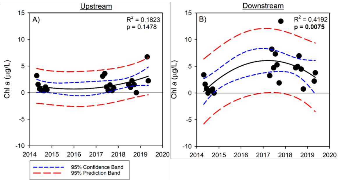
Figure 6. Bear Creek chlorophyll a regressions at Upstream (A) and Downstream (B) sites. Legend below A applies to both panels. Significant ( p < 0.05 ) regression ANOVA p -values are noted in bold text.
