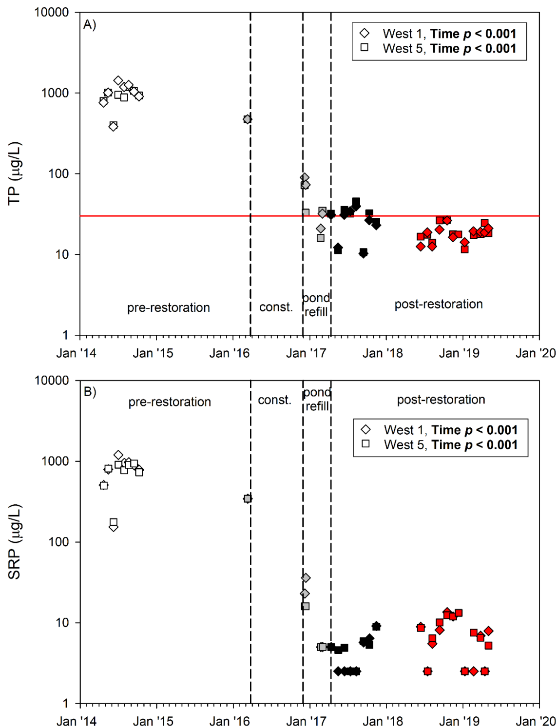
Figure 9. West pond TP (A) and SRP (B) site concentrations over entire 2014-2019 monitoring period. P-values in the inserted boxes compare only 2014 pre-restoration (white) and the most recent 2018-19 post-restoration data (red symbols) as paired t-tests matched by sampling month (Table 5). Restoration construction (grey), pond refill (grey), and the first year of post-restoration (black) samples are not included in this statistical analysis. Red reference line at 30 µg/L represents TP target goal set by the Bear Lake TMDL (MDEQ 2008). Note the log scale y-axis.
