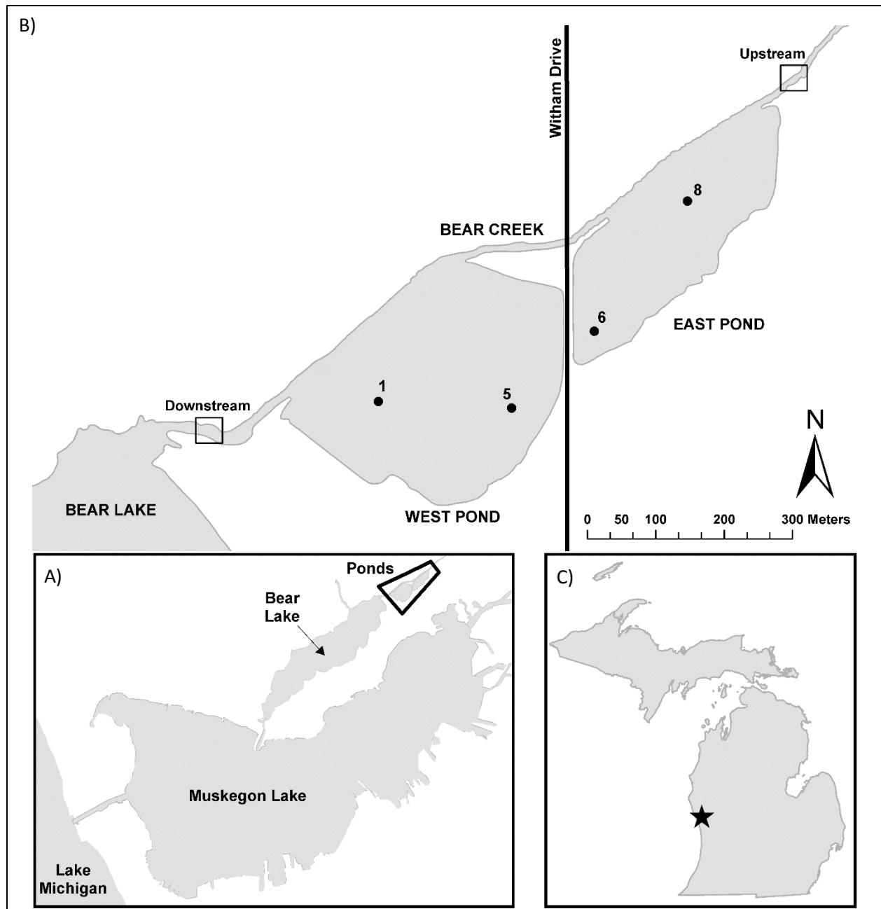
Figure 1. A) location of restoration area (outlined in thick black lines) within the Muskegon Lake Area of Concern; B) magnified view of restoration site, including the reconnected ponds and Bear Creek, and C) location of Muskegon (star) in map of Michigan. Note that this figure uses map outlines from pre-restoration (2016) satellite imagery. Official satellite imagery captured after restoration construction occurred was not yet released as of June 2019. The pre-restoration pond outlines shown here are edited to represent that the earthen berms previously separating ponds from Bear Creek have been removed.
