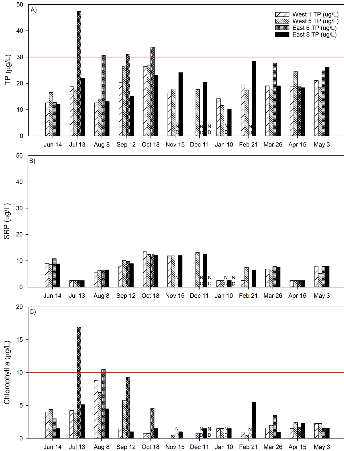
Figure 7. Post-restoration (June 2018 through May 2019) TP, SRP, and chl a concentrations at West and East pond sites. Red reference lines at 30 and 10 µg/L represent the TP target goal set by the Bear Lake TMDL (MDEQ 2008) and chl a restoration goal for Muskegon Lake AOC, respectively. ND = no data for pond sites that couldn't be safely sampled during winter 2018-19 (Table 1).
