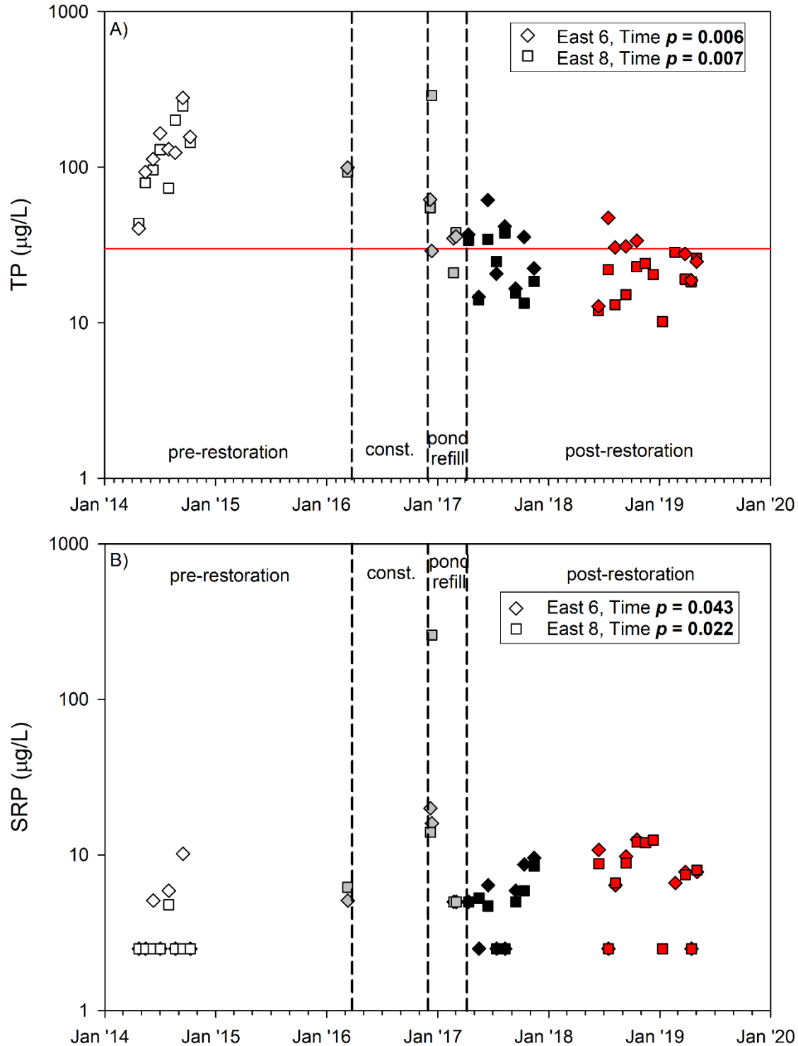
Figure 12. East pond TP (A) and SRP (B) site concentrations over entire 2014-2019 monitoring period. P-values in the inserted boxes compare only pre-restoration (white) and the most recent 2018-19 post-restoration data (red symbols) as paired t-tests matched by sampling month (Table 7). Restoration construction (grey), pond refill (grey), and the first year of post-restoration (black) samples are not included in this statistical analysis. Red reference line at 30 µg/L represents TP target goal set by the Bear Lake TMDL (MDEQ 2008). Note the log scale y-axis.
