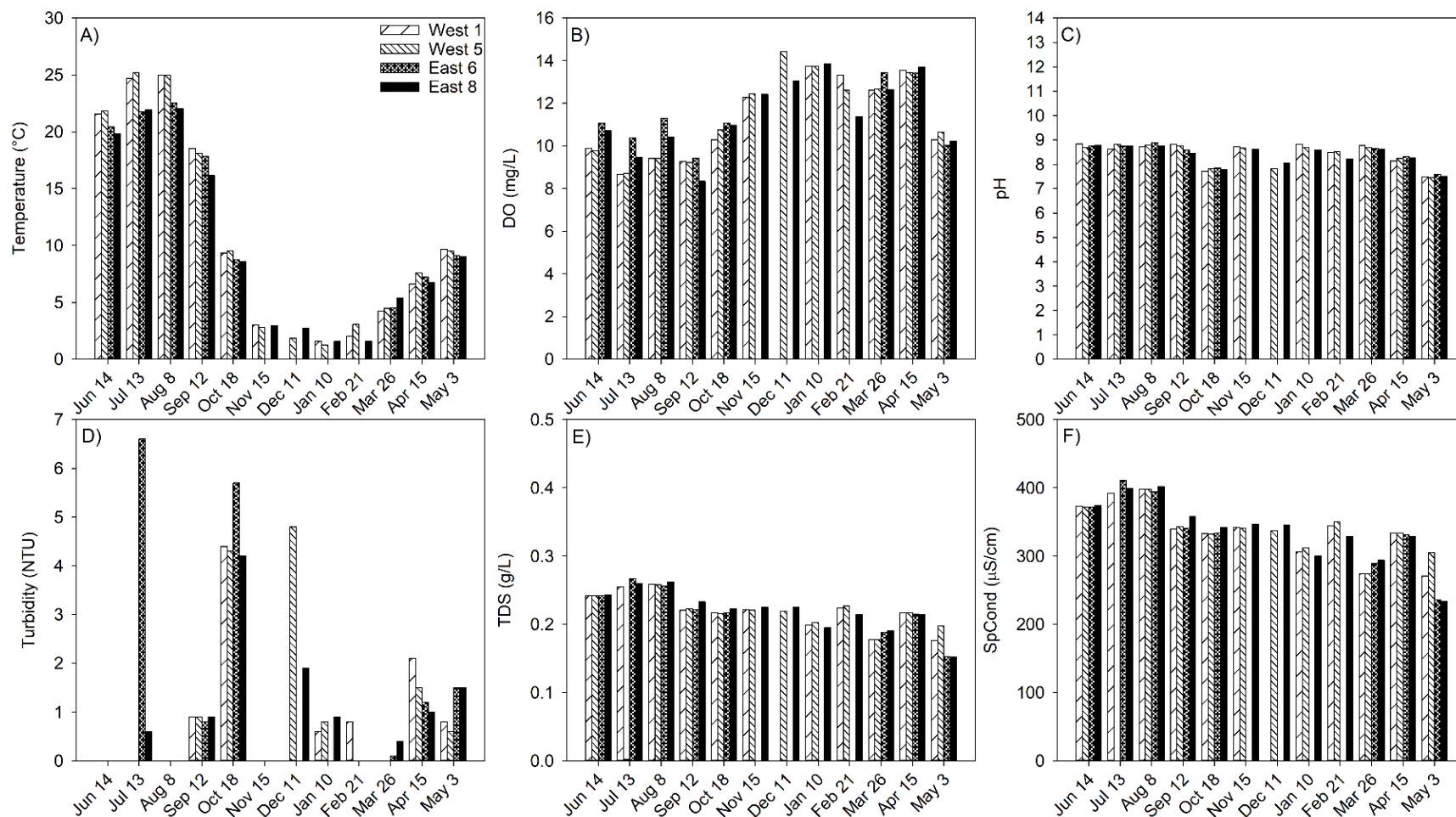
Figure 8. Temperature, dissolved oxygen (DO), pH, turbidity, total dissolved solids (TDS), and specific conductivity (SpCond) of West and East pond sites after wetland restoration (June 2018 – May 2019). See Table 1 for a description of when pond sites couldn't be safely sampled during winter 2018-19, resulting in no data.
