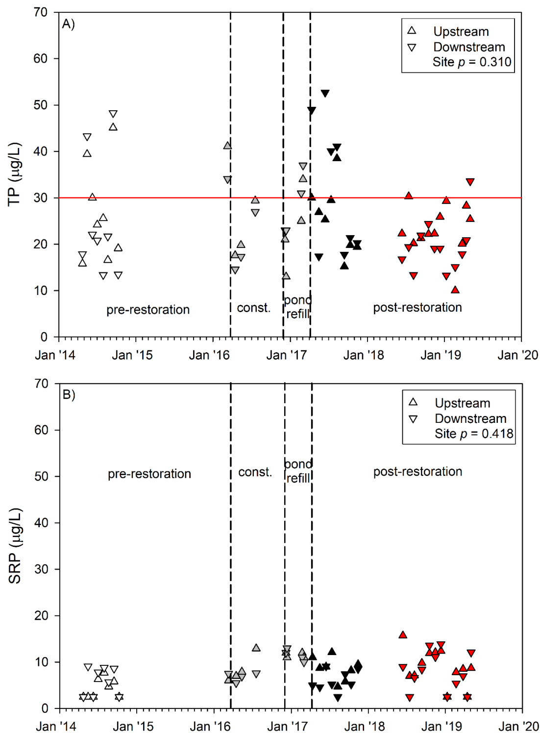
Figure 4. Bear Creek TP (A) and SRP (B) site concentrations over entire 2014-2019 monitoring period. P-values in the inserted boxes are based on only the post-restoration data (red symbols), comparing 2018-19 monthly upstream vs. downstream paired t-tests (Table 3). Pre-restoration (white and one set of grey symbols), construction (grey), pond refill (grey), and the first year of post-restoration (black) samples are not included in this statistical analysis. Red reference line at 30 µg/L represents TP target goal set by the Bear Lake TMDL (MDEQ 2008).
