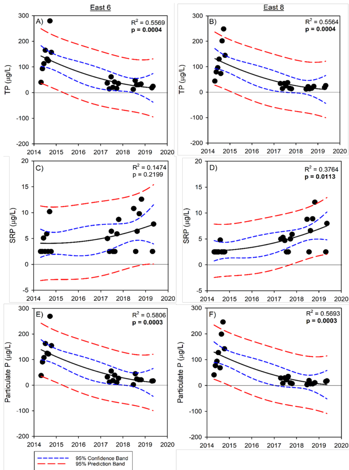
Figure 13. East pond phosphorus regressions of TP (A-B), SRP, (C-D), and particulate P (E-F) at sites East 6 (A, C, E) and East 8 (B, D, F). Legend below E applies to all panels. Significant ( p < 0.05 ) regression ANOVA p -values are noted in bold text.
