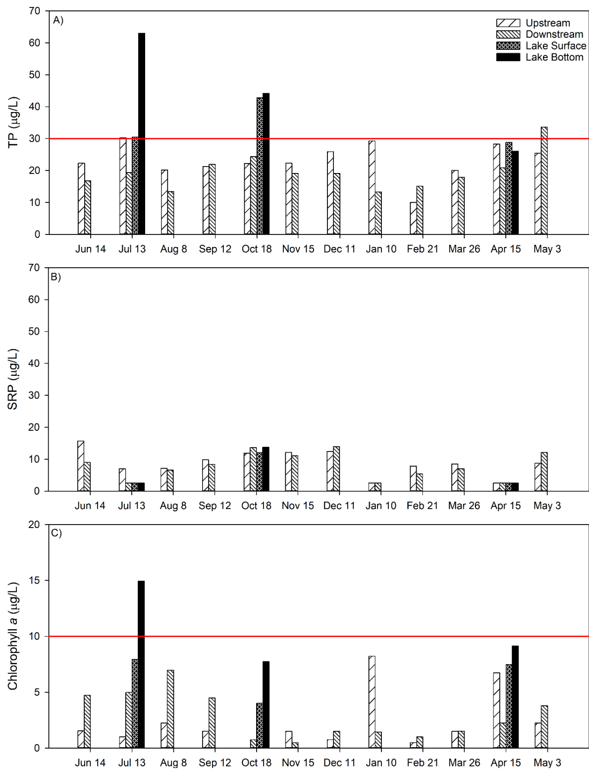
Figure 2. Post-restoration (June 2018 through May 2019) TP, SRP, and chl a concentrations at Bear Creek and Bear Lake sites. Bear Lake sites were sampled only in July and October 2018 and in April 2019. Red reference lines at 30 and 10 µg/L represent the TP target goal set by the Bear Lake TMDL (MDEQ 2008) and chl a restoration goal for Muskegon Lake AOC, respectively.
