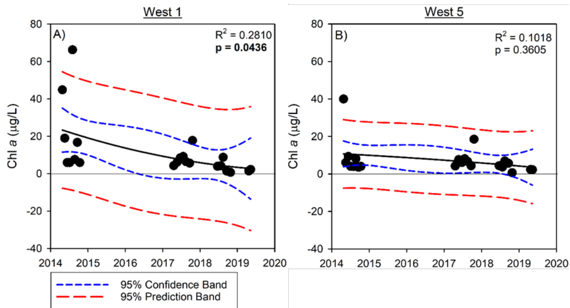
Figure 11. West pond chlorophyll a regressions at sites West 1 (A) and West 5 (B). Legend below A applies to both panels. Significant ( p < 0.05 ) regression ANOVA p -values are noted in bold text.
