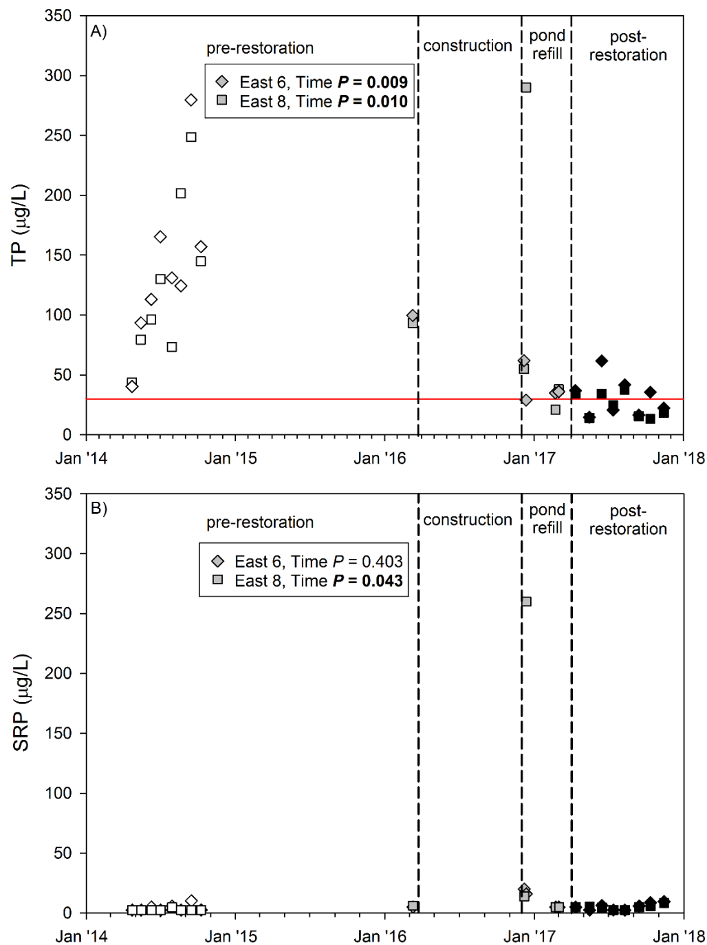
Figure 8. East pond TP (A) and SRP (B) site concentrations during 2014-2016 pre-restoration sampling and 2017 post-restoration sampling. P-values are results of pre- vs. post-restoration paired t-tests within sites. Pond refill samples (gray symbols) are not included in statistical analysis. Red reference lines at 30 µg/L represent TP target goal set by the Bear Lake TMDL (MDEQ 2008).
