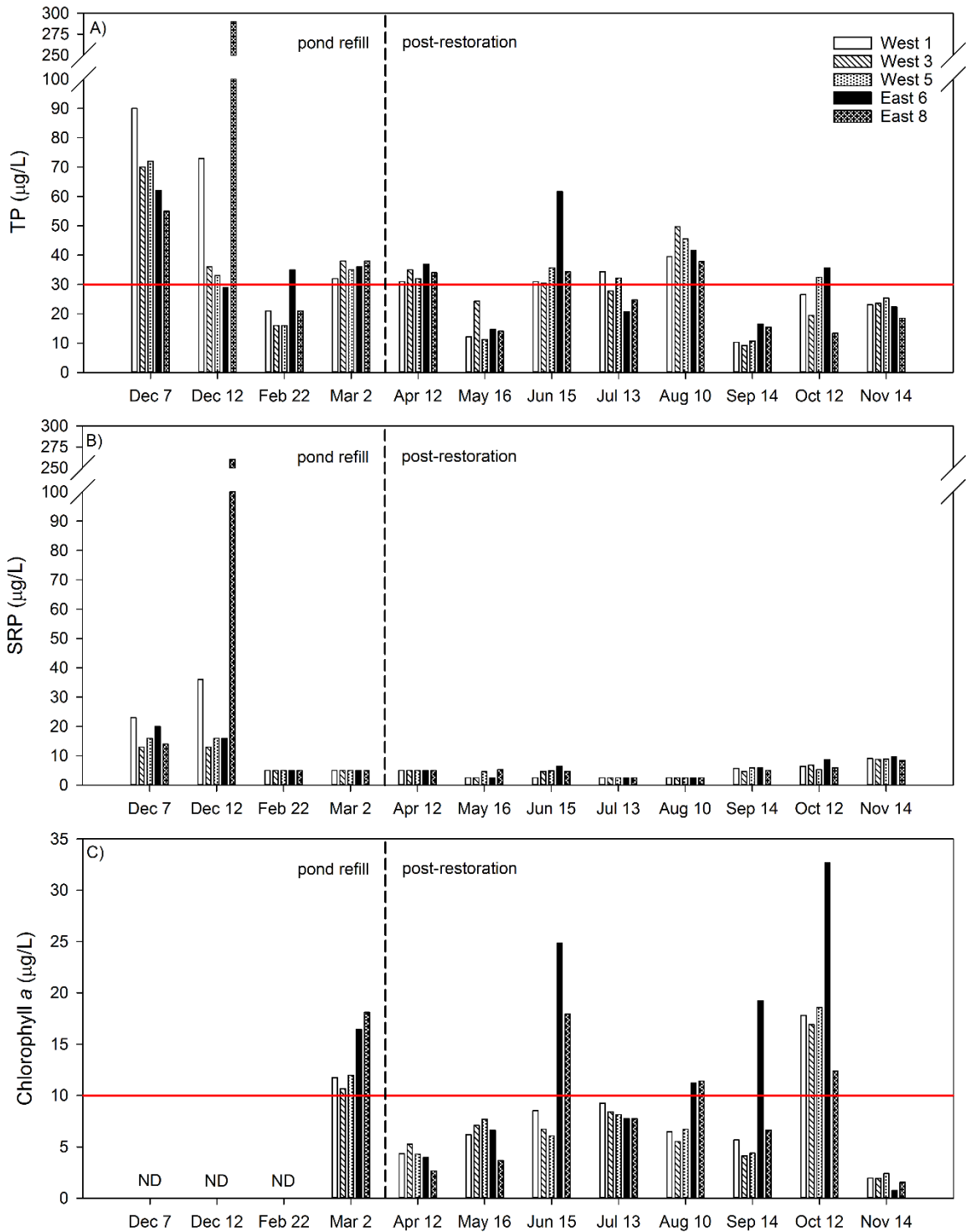
Figure 5. December 2016 through November 2017 TP (A), SRP (B), and chlorophyll (C) site concentrations at West and East ponds. Note that y-axis scales differ among panels and that y-axes in panels A and B are broken and that axis scales before and after the breaks are not identical. ND = no data, as chlorophyll was not sampled during winter 2016-2017. Red reference lines at 30 and 10 µg/L represent TP target goal set by the Bear Lake TMDL (MDEQ 2008) and chl restoration goal for Muskegon Lake AOC, respectively.
