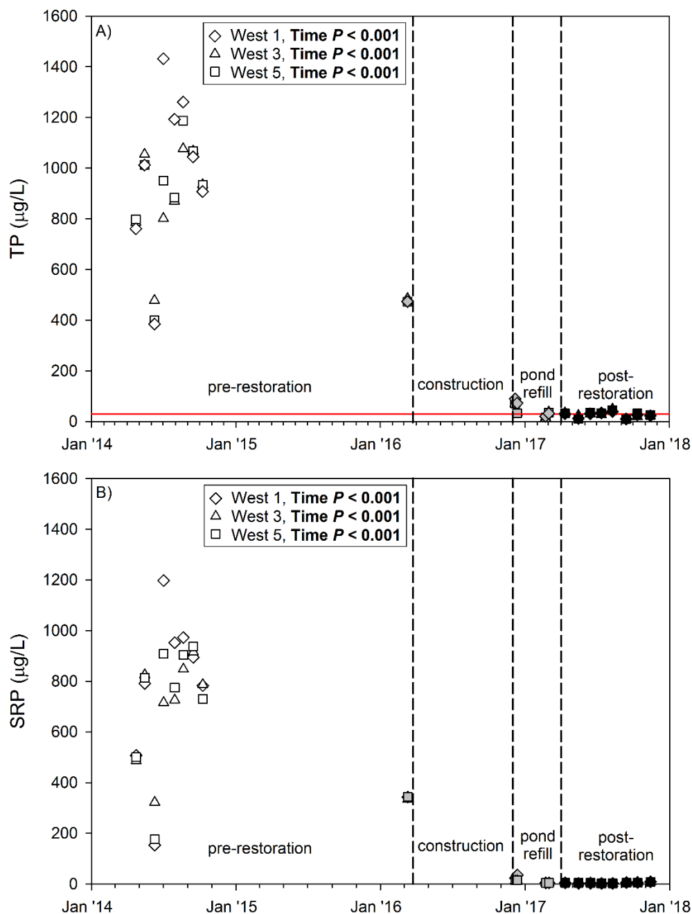
Figure 7. West pond TP (A) and SRP (B) site concentrations during 2014-2016 pre-restoration sampling and 2017 post-restoration sampling. P-values are results of pre- vs. post-restoration paired t-tests within sites. Pond refill samples (gray symbols) are not included in statistical analysis. Red reference lines at 30 µg/L represent TP target goal set by the Bear Lake TMDL (MDEQ 2008).
