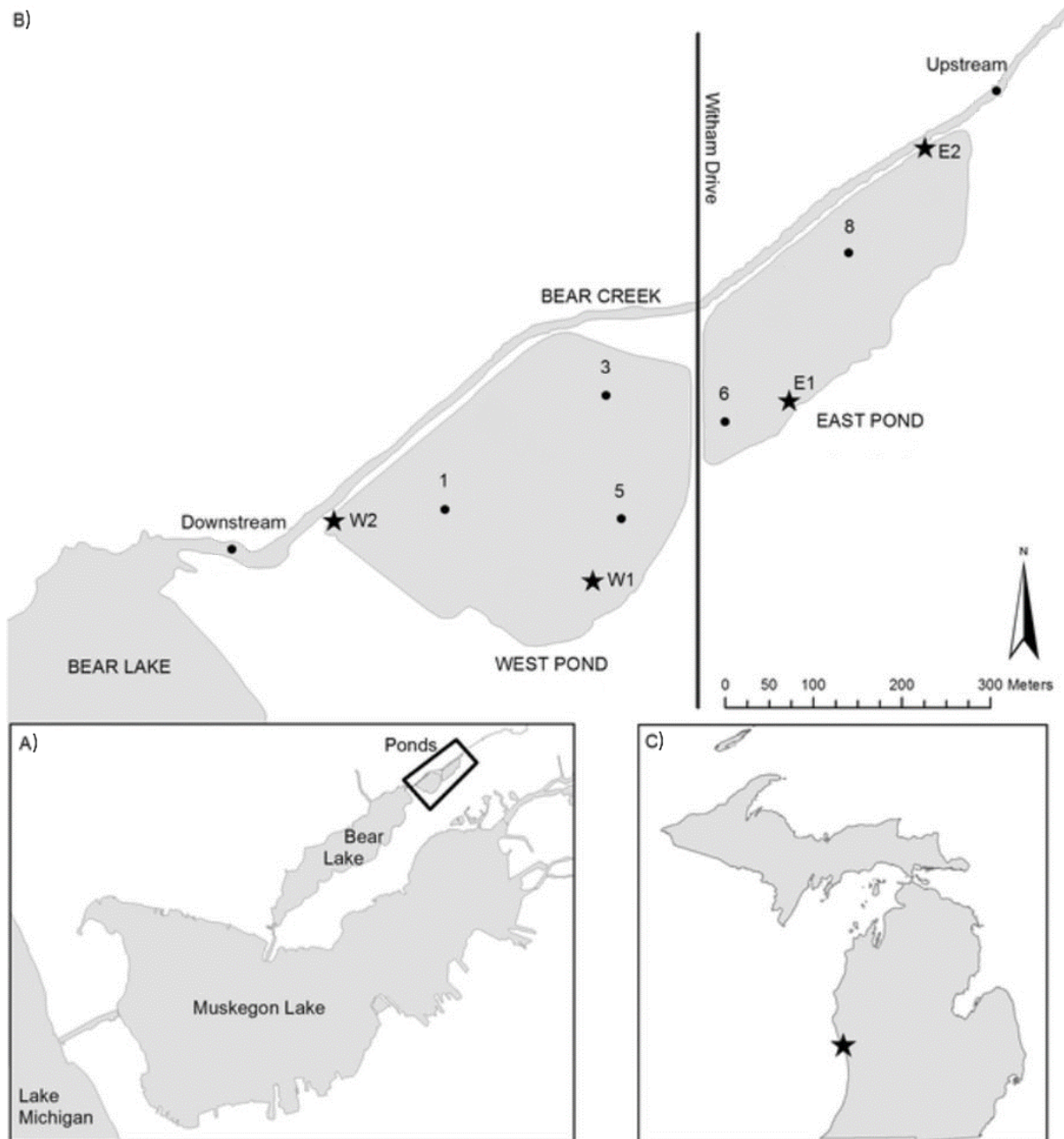
Figure 1. A) location of restoration area (outlined in thick black lines) within the Muskegon Lake Area of Concern; B) blow up of restoration site, including the two ponds that were dredged, Bear Creek, and sampling locations for water quality and sediment isotherms (dots) and sediment porewater (stars); and C) location of Muskegon (star) in map of Michigan. Note that this map uses outlines from pre-restoration satellite imagery; the earthen berm that previously separated the ponds from Bear Creek has been removed.
