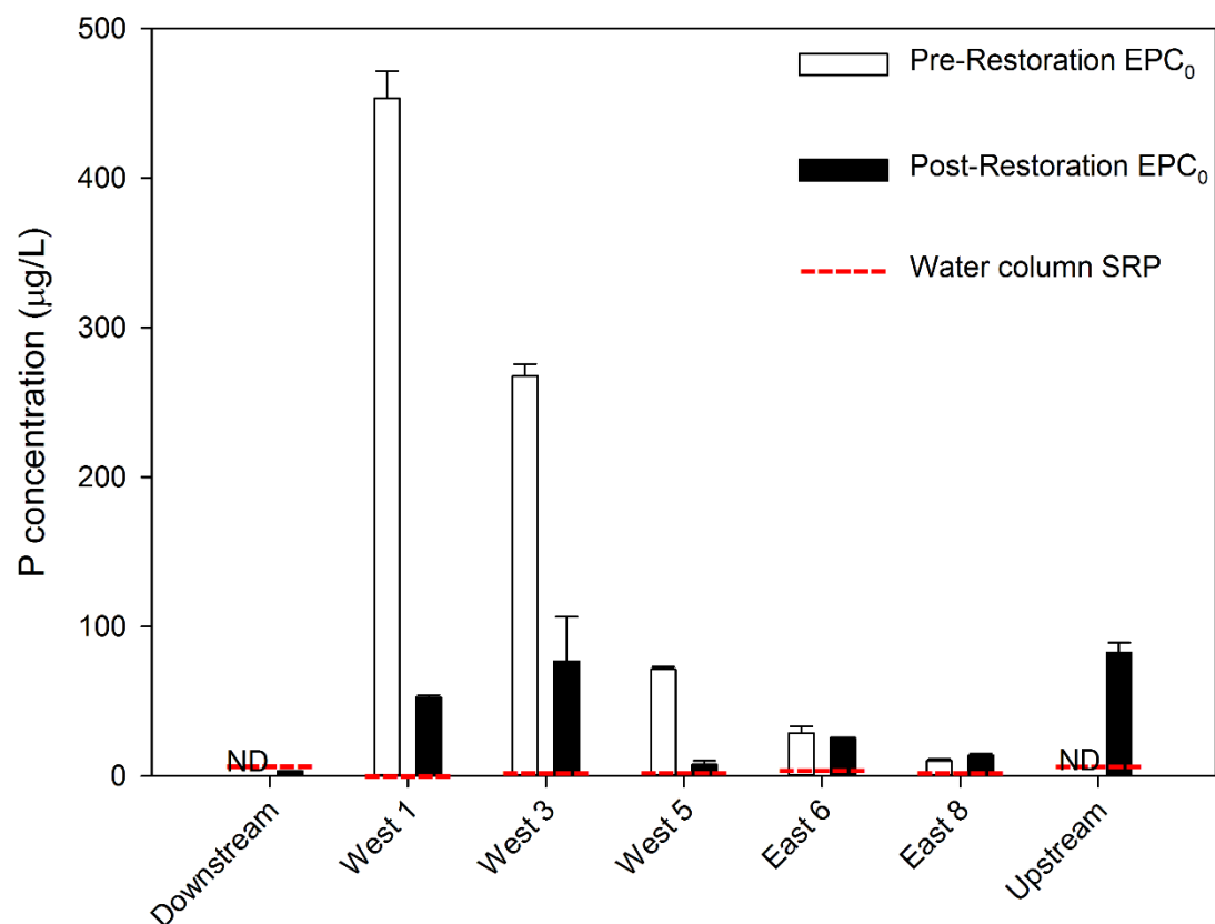
Figure 9. Sediment P isotherm data for pre-restoration (18 July 2012) and post-restoration (27-28 June 2017) sampling events at Bear Creek and pond sites. Red dashed lines represent water column SRP concentrations collected in June 2017. ND=no data (as sediment was not collected from Bear Creek sites for isotherm analysis in 2012).
