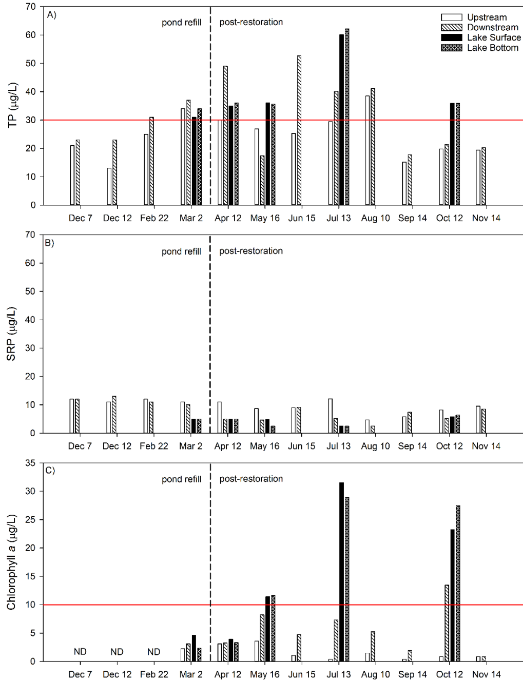
Figure 2. Post-dredging (December 2016 through November 2017) TP, SRP, and chl a concentrations at Bear Creek and Bear Lake sites. Bear Lake sites post-dredging were sampled only in March-May, July, and October 2017. ND = no data, as chlorophyll was not sampled during winter 2016-2017. Red reference lines at 30 and 10 µg/L represent the TP target goal set by the Bear Lake TMDL (MDEQ 2008) and chl a restoration goal for Muskegon Lake AOC, respectively.
