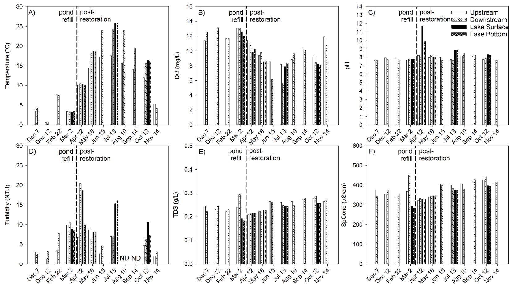
Figure 3. Temperature, dissolved oxygen (DO), pH, turbidity, total dissolved solids (TDS), and specific conductance (SpCond) of Bear Creek upstream & downstream and Bear Lake near-surface and near-bottom sites during pond refill (Dec. 2016 – Mar. 2017), berm removal (Apr. 2017), and post-filling (May – Nov. 2017) periods. Bear Lake sites post-restoration were sampled only in Mar.-May, Jul., and Oct. 2017. ND = no data (due to turbidity sensor error in August and September).
