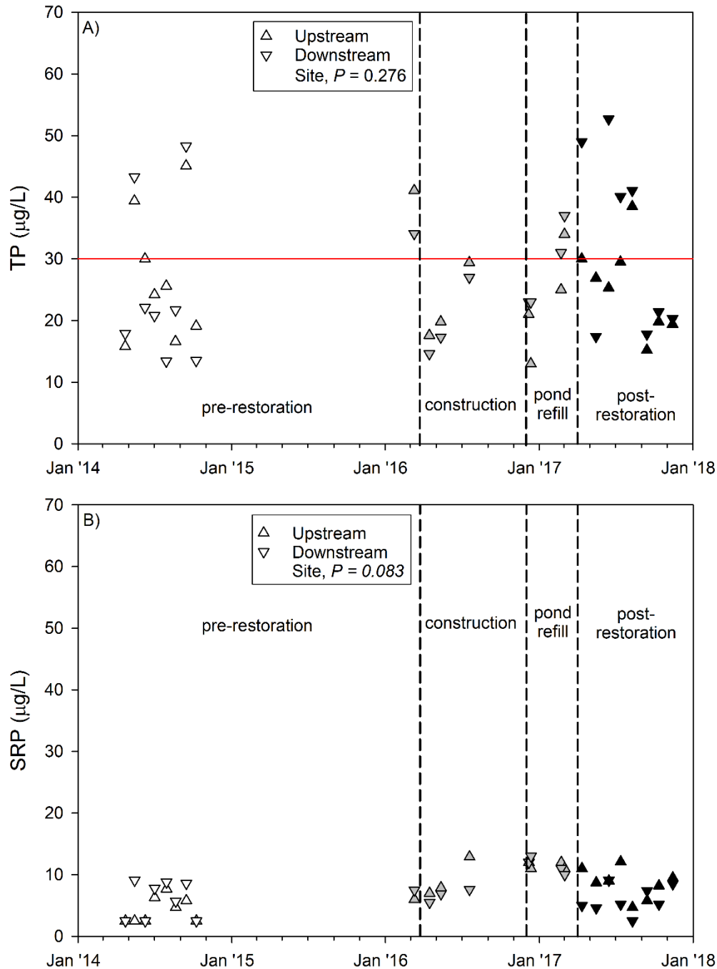
Figure 4. Bear Creek TP (A) and SRP (B) site concentrations over project period. P-values in the inserted boxes are based on only the post-restoration data (black symbols), comparing monthly upstream vs. downstream paired t-tests. Pre-restoration (open and one set of grey symbols), construction (grey symbols), and pond refill (grey symbols) samples are not included in this statistical analysis. Red reference line at 30 µg/L represents TP target goal set by the Bear Lake TMDL (MDEQ 2008).
