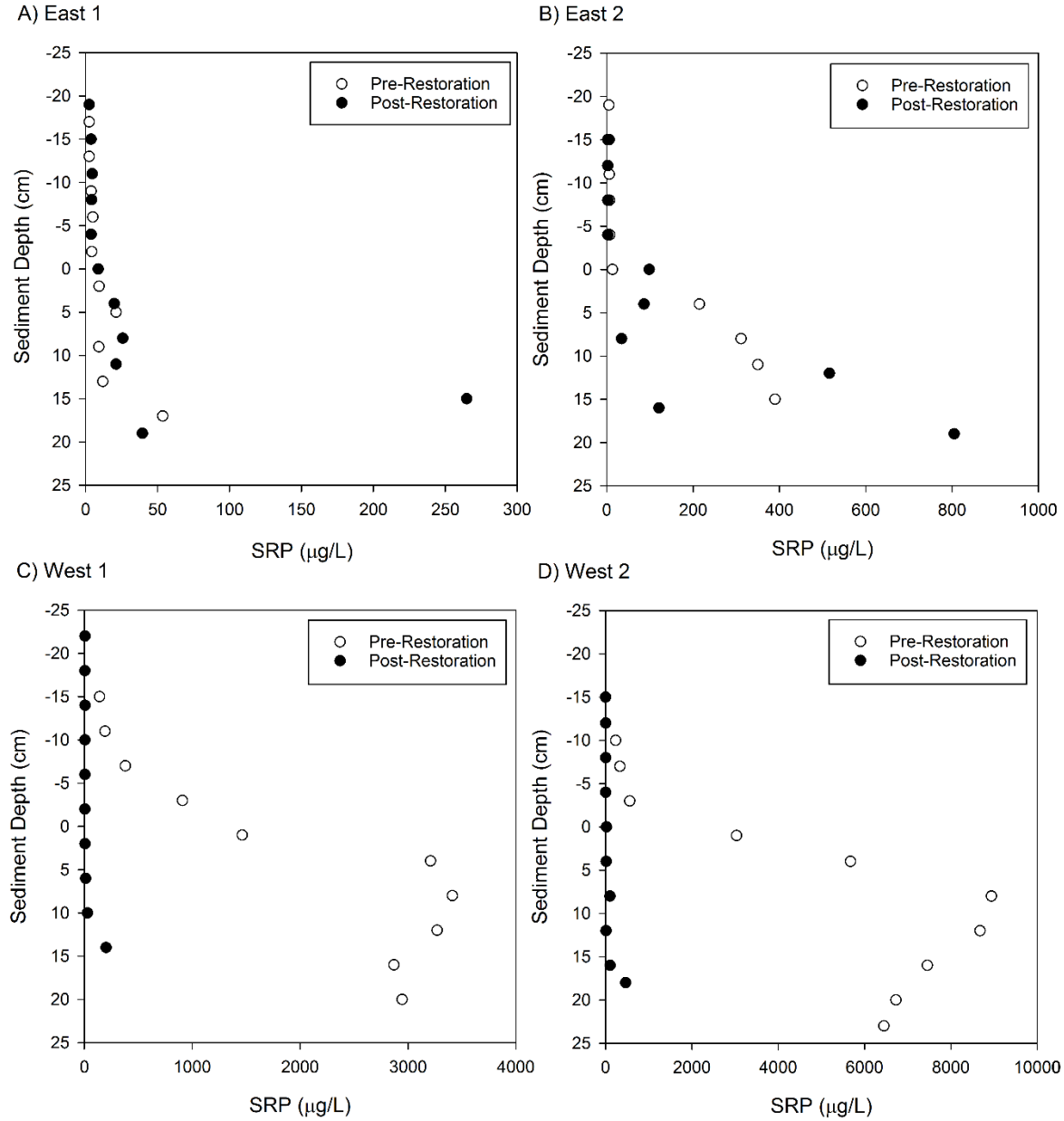
Figure 10. Pre- and post-restoration mean sediment porewater P by depth in restoration ponds. For each site, n=2 porewater sampling units. Pre-restoration peepers incubated in situ 18 July 2012 to 1 August 2012 and post-restoration peepers incubated in situ 31 August 2017 to 14 September 2017.
