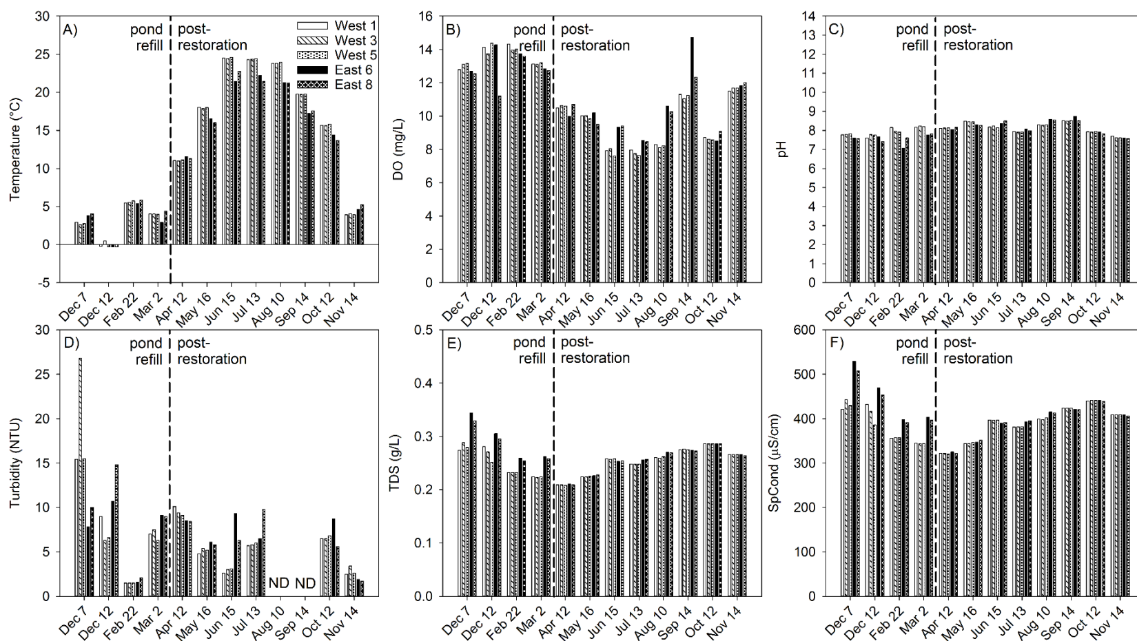
Figure 6. Temperature, dissolved oxygen (DO), pH, turbidity, total dissolved solids (TDS), and specific conductance (SpCond) of West and East pond sites during pond refill (Dec. 2016 – Mar. 2017), berm removal (Apr. 2017), and post-filling (May – Nov. 2017) periods. ND = no data (due to turbidity sensor error in August and September).
