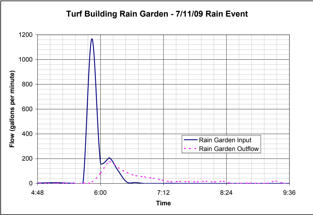
Graph of water flow into and out of the rain garden during a storm event 7/11/09
