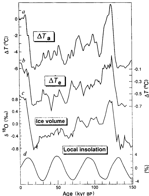
FIG. 3 Time series of the Vostok climate record and of climate forcings used in the multivariate analysis: a, atmospheric temperature change over Antarctica (Vostok record), \Delta T_a ; b, the direct greenhouse radiative forcing accounting for \text{CO}_2 and \text{CH}_4 variations, \Delta T_e ; c, \delta^{18}\text{O} SPECMAP record taken as a proxy of the change in ice volume (normalized value from ref. 33); d, percentage change in total insolation at the Vostok latitude ( 78^\circ\text{S} ) during the entire year. Vostok curves (a and b) have been redated for the period before 110 kyr in such a way to put the Vostok temperature and the marine records in phase.
