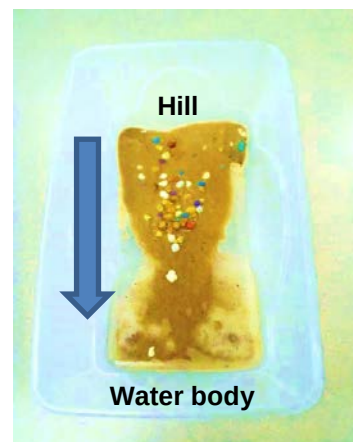
Sample model of a stream (J.Vail)
