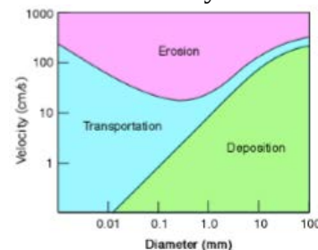
Hjulstrom's Diagram http://www.columbia.edu/~vjd1/streams_basic.htm
