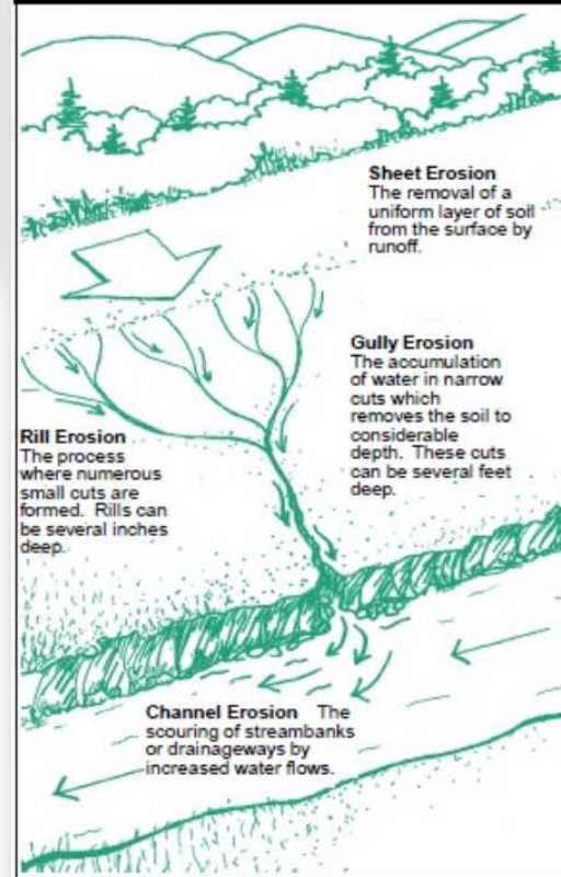
Types of Erosion http://www.fairfaxcounty.gov/nvswcd/youyourland/soil.htm
