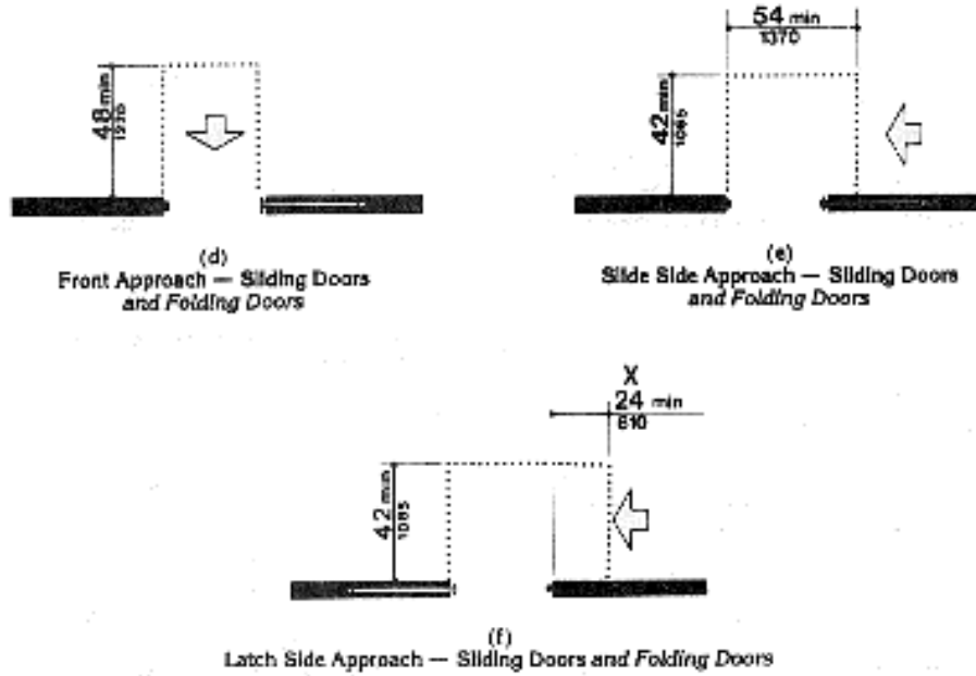
Figure 25 (4.13.6) Maneuvering Clearances at Doors
