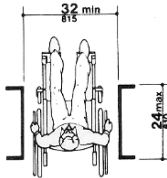
Figure 24e (4.13.5) Clear Doorway Width and Depth Maximum Doorway Depth
