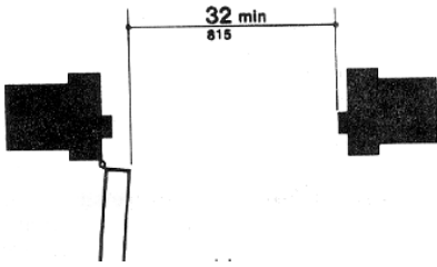
Figure 24a (4.13.5) Clear Doorway Width and Depth Detail
