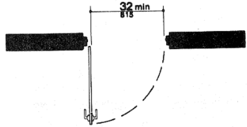
Figure 24b (4.13.5) Clear Doorway Width and Depth Hinged Door
