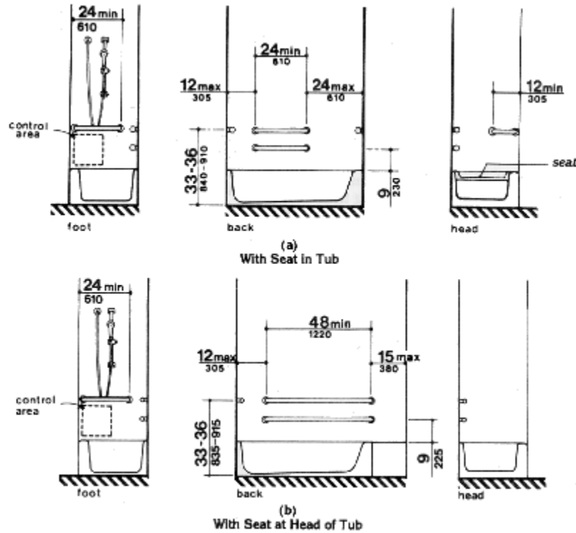
Figure 34 (4.20) Grab Bars at Bathtubs
