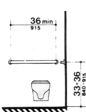
Figure 30c (4.17.6) Toilet Stalls Rear Wall of Standard Stall
