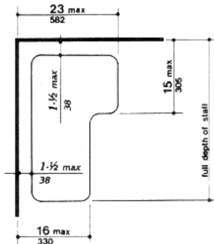
Figure 36 (4.21.3) Shower Seat Design
