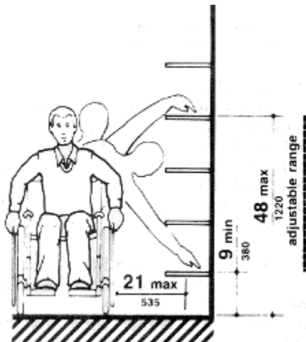
Figure 38a (4.25.3)
