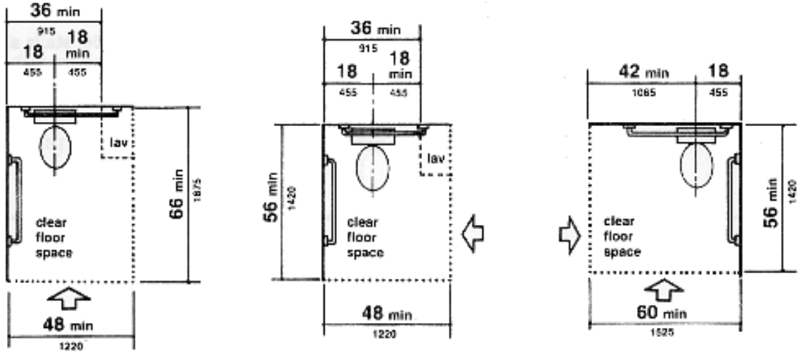
Figure 28 (4.16.2) Clear Floor Space at Water Closets
