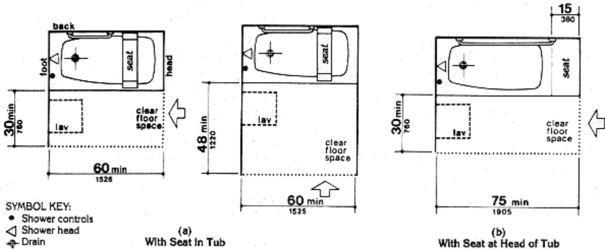
Figure 33 (4.20) Clear Space at Bathtubs
