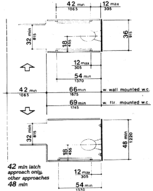
Figure 30b(4.17.6) Toilet Stalls Alternate Stalls
