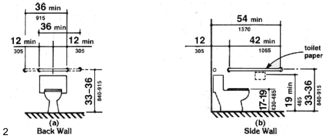
Figure 29 (4.16.4) Grab Bars at Water Closets
