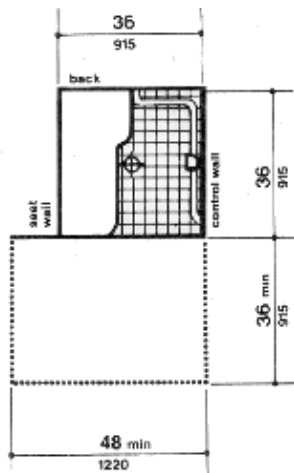
Figure 35a (4.21.2)
