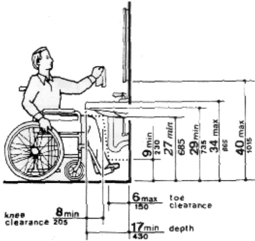
Figure 31 (4.19) Lavatory Clearances
