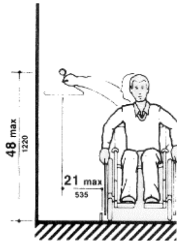
Figure 38b (4.25.3)
