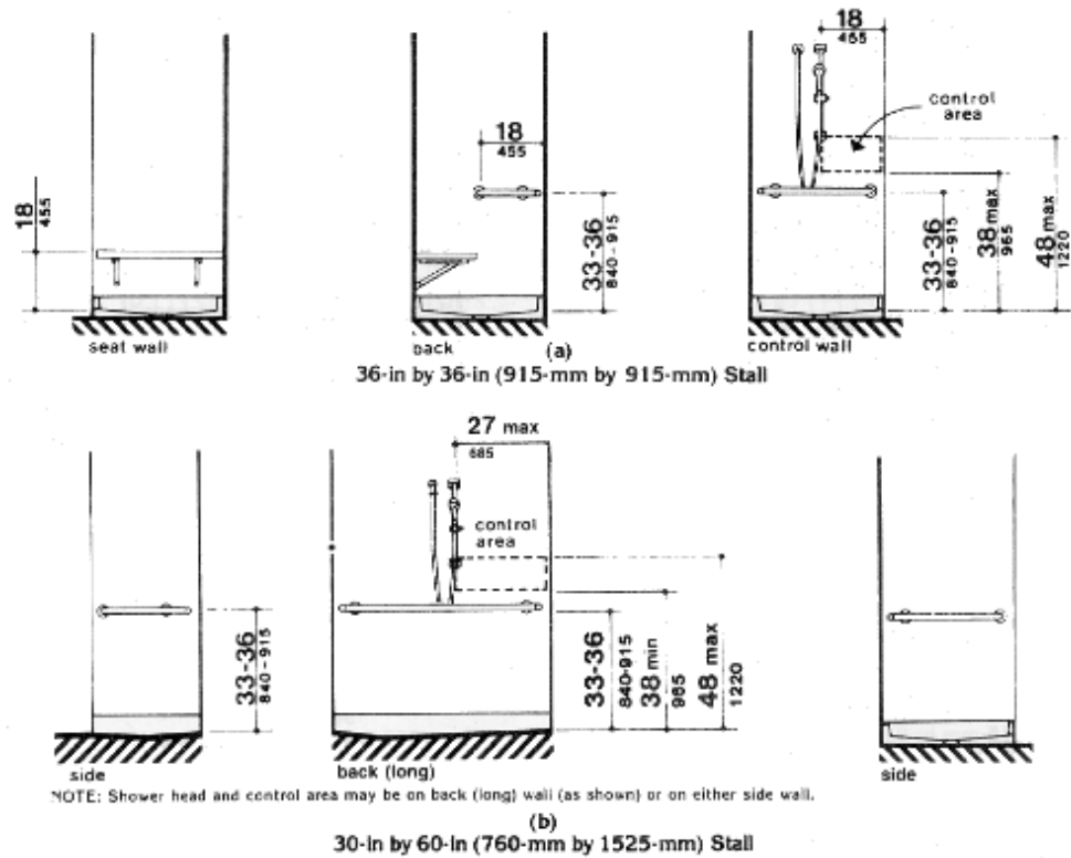
Figure 37 (4.21) Grab Bars at Shower Stalls
