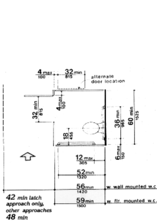
Figure 30a (4.17.6) Toilet Stalls Standard Stall
