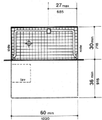
Figure 35b (4.21.2)
