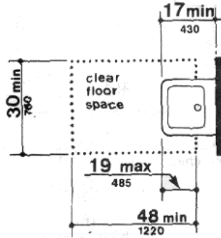
Figure 32 (4.19) Clear Floor Space at Lavatories
