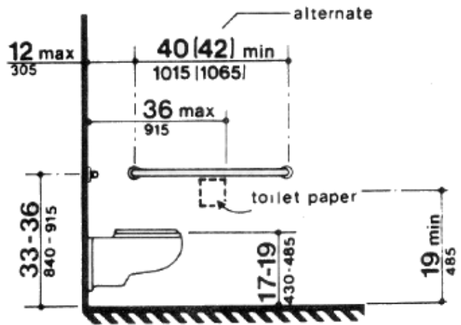
Figure 30d (4.17.6) Toilet Stalls
