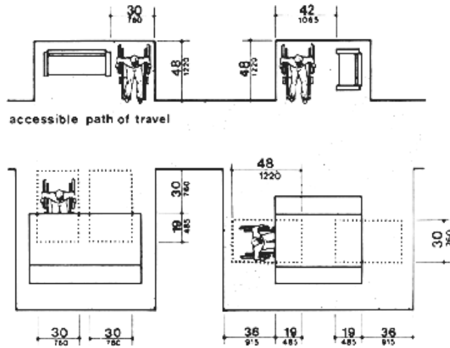
Fig. 45 Minimum Clearances for Seating and Tables
