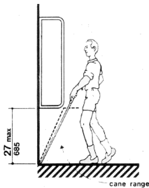
Figure 8b ( 4.4.1) Protruding Objects Walking Perpendicular to a Wall
