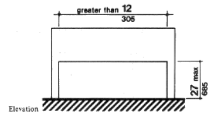
Figure 8c ( 4.4.1) Protruding Objects Free-Standing Overhanging Objects
