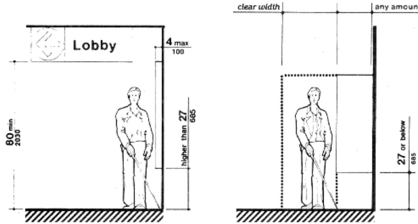
Figure 8a ( 4.4.1) Protruding Objects Walking Parallel to a Wall
