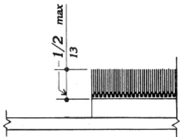
Figure 8F (4.5.3) Carpet Pile Thickness
