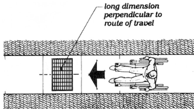
Figure 8h (4.5.4) Gratings Orientation
