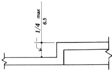
Figure 7(c) (4.5.2) Accessible Route - Changes in level
