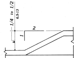
Figure 7(d) (4.5.2) Accessible Route - Changes in level
